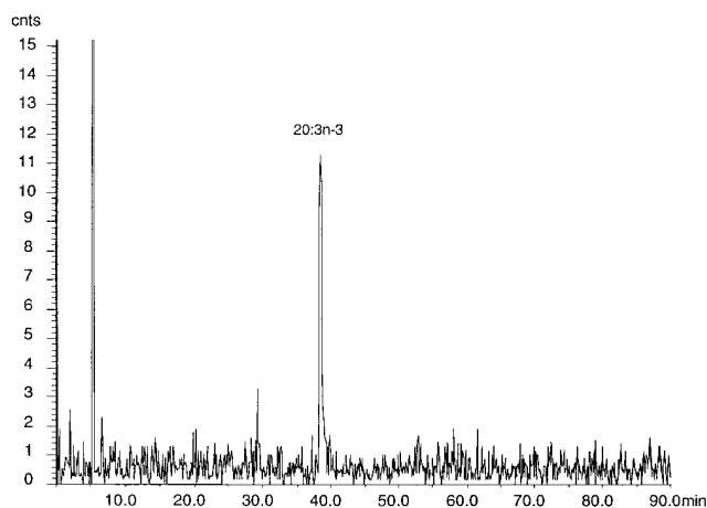
Fig. 5. Radiochromatograms of labeled metabolites produced from [1- 14 C]α-linolenic acid in 2-h post-perfused rat liver. Top: in the first HPLC fraction (F1). Bottom: in the third HPLC fraction (F3).
